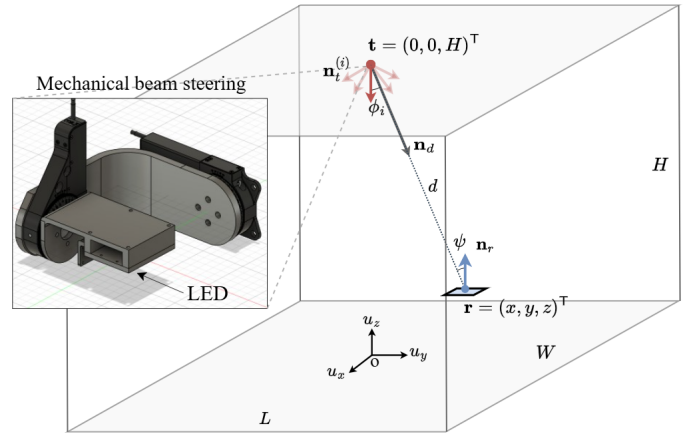
Fig. 1. Configuration of the system single-LED Optical Wireless Positioning.
